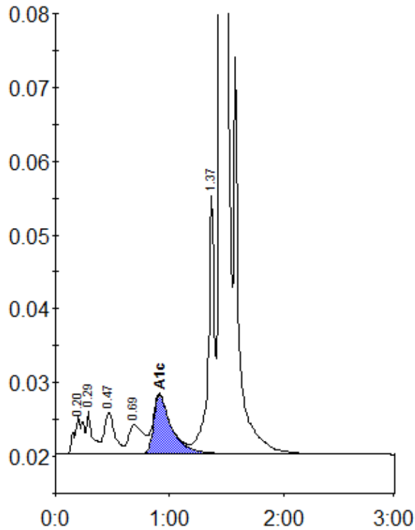
Peak table - ID: 10399612
